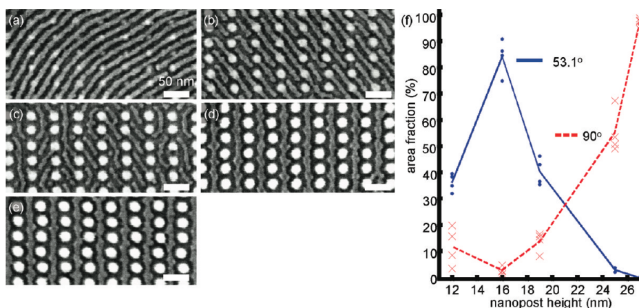
Figure 3. SEM images of PDMS microdomains templated by post arrays with various heights. L_x and L_y of the array was 48 and 32 nm, respectively. The diameter of posts was 12 nm, and the height of posts was (a) 12, (b) 16, (c) 19, (d) 25, and (e) 27 nm. Scale bar = 50 nm. (f) The area fractions of the cylinders oriented along the commensurate orientation and the y-axis. Each set of post height data came from a separate sample. (a–e) The samples were slightly overetched, which makes the PDMS cylinders disconnected.
